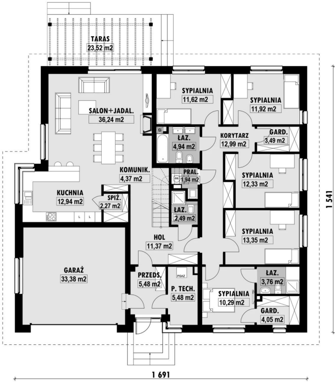
E-246 PARTER E-246 PARTER
