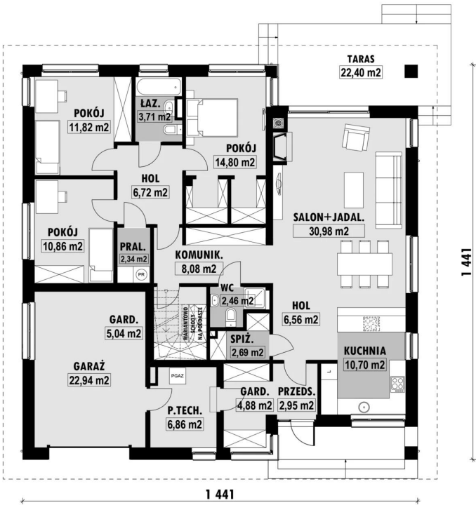
E-240 PARTER E-240 PARTER
