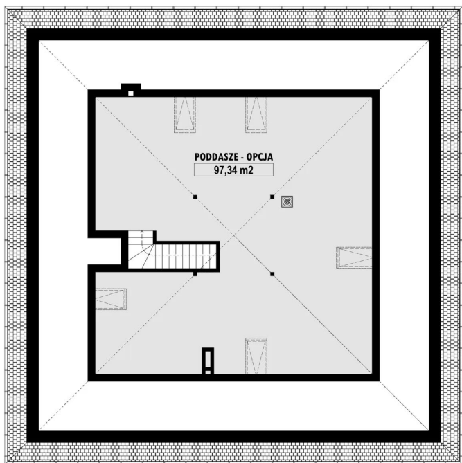
E-235 PODDASZE E-235 PODDASZE
