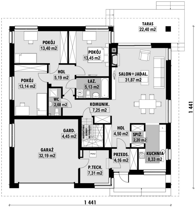
E-230 PARTER E-230 PARTER
