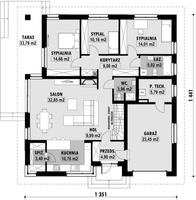
E-227 PARTER E-227 PARTER
