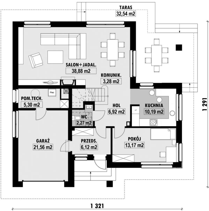
E-168 PARTER E-168 PARTER
