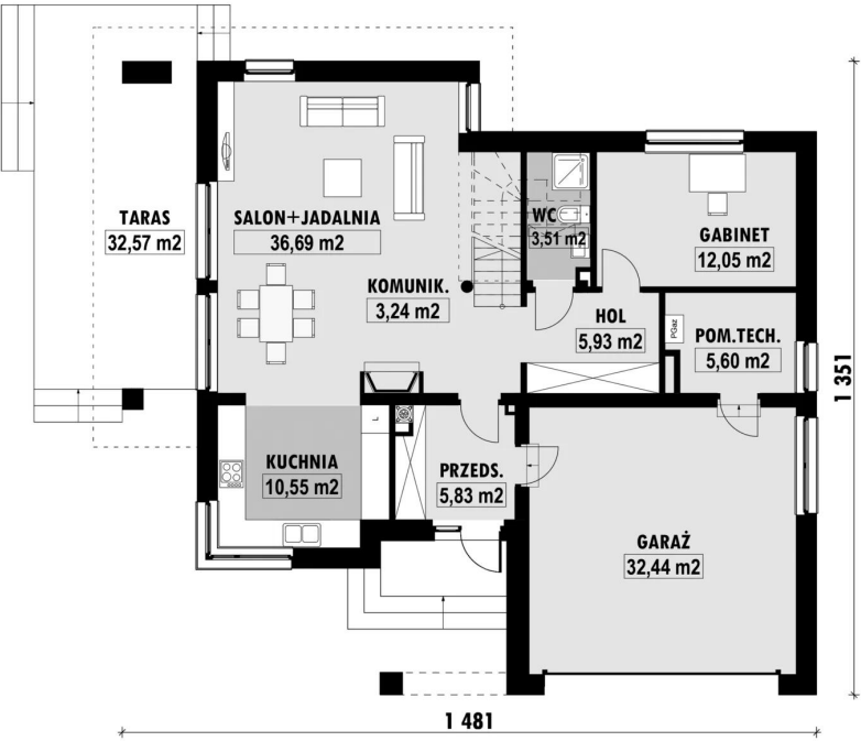
E-166a PARTER E-166a PARTER
