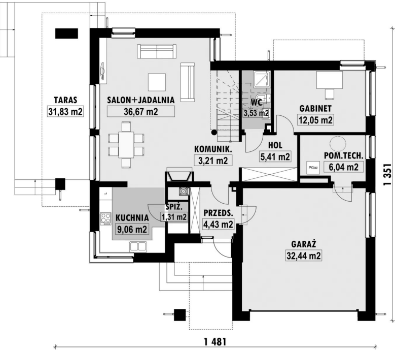
E-166 PARTER E-166 PARTER
