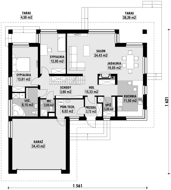
E-155 PARTER E-155 PARTER
