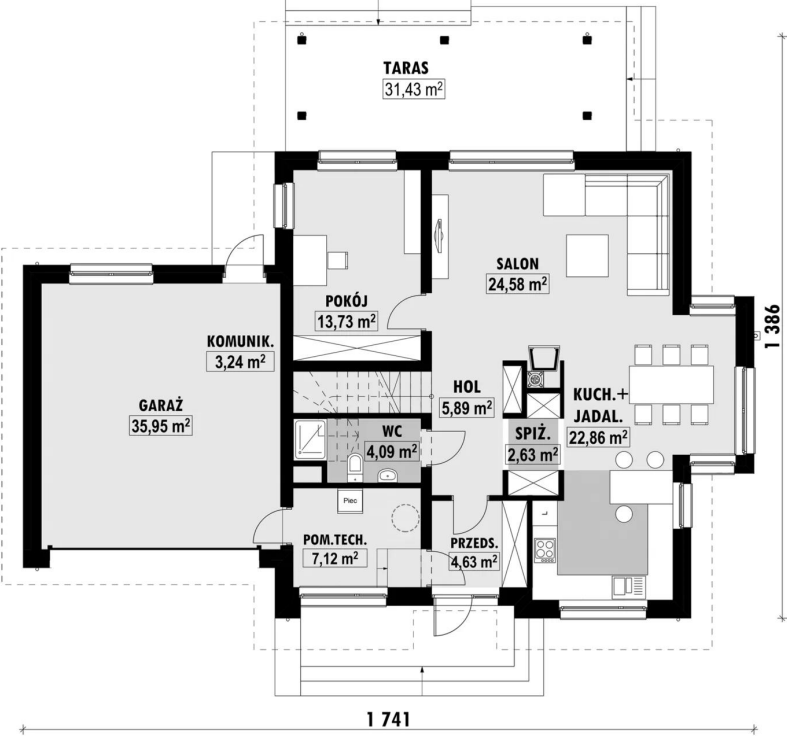
E-147 PARTER E-147 PARTER
