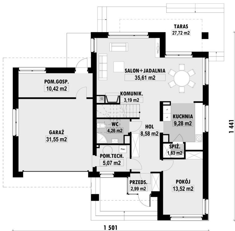
E-130 PARTER E-130 PARTER
