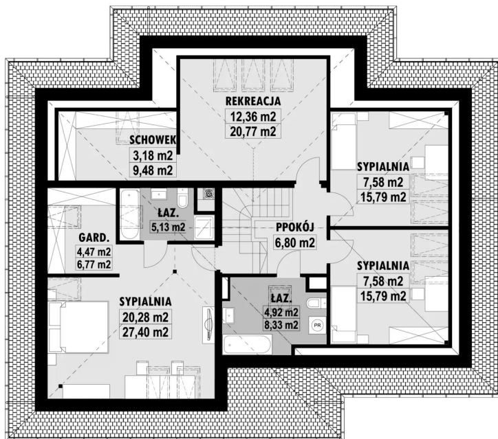
E-128 PODDASZE E-128 PODDASZE
