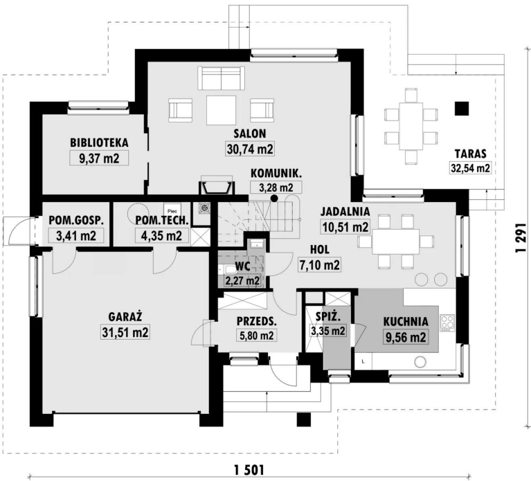
E-128 PARTER E-128 PARTER
