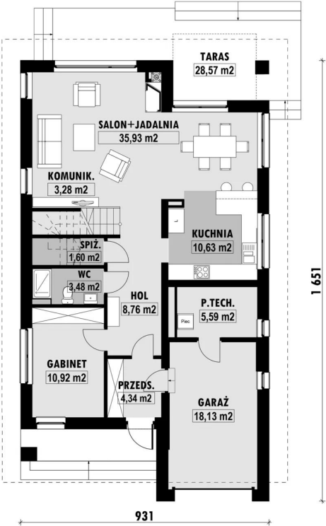
E-107a PARTER E-107a PARTER
