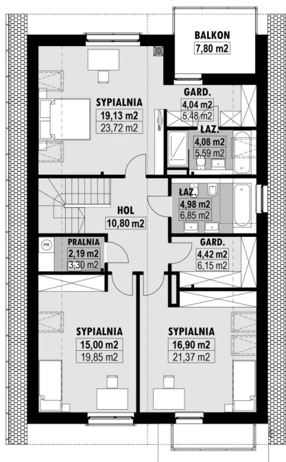
E-107a PODDASZE E-107a PODDASZE
