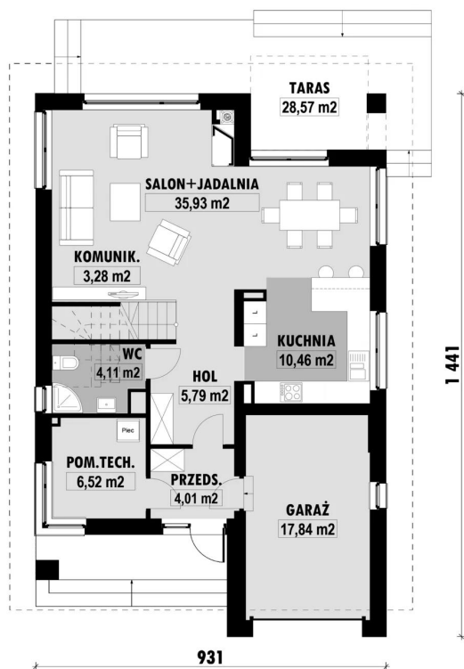
E-107 PARTER E-107 PARTER
