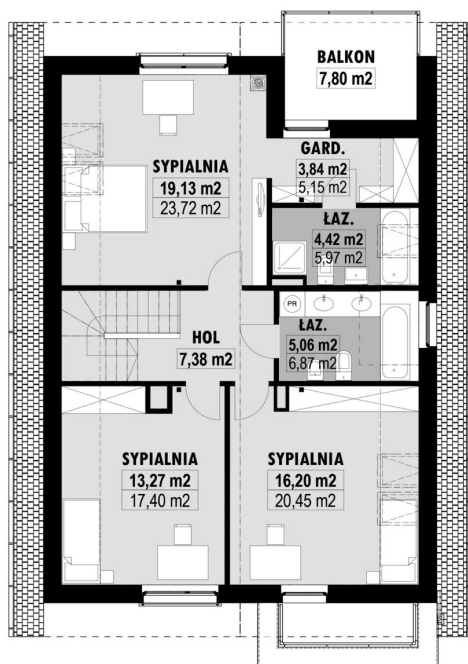
E-107 PODDASZE E-107 PODDASZE
