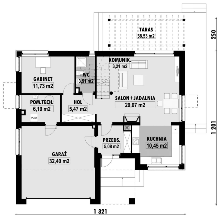
E-102 PARTER E-102 PARTER
