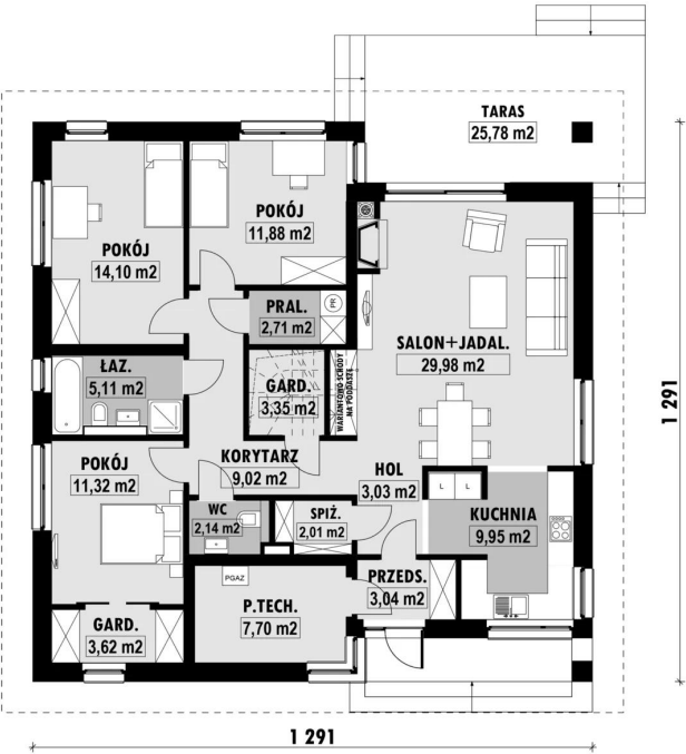
E-269 PARTER E-269 PARTER
