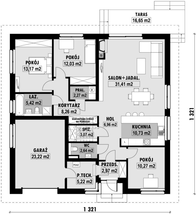
E-268 PARTER E-268 PARTER
